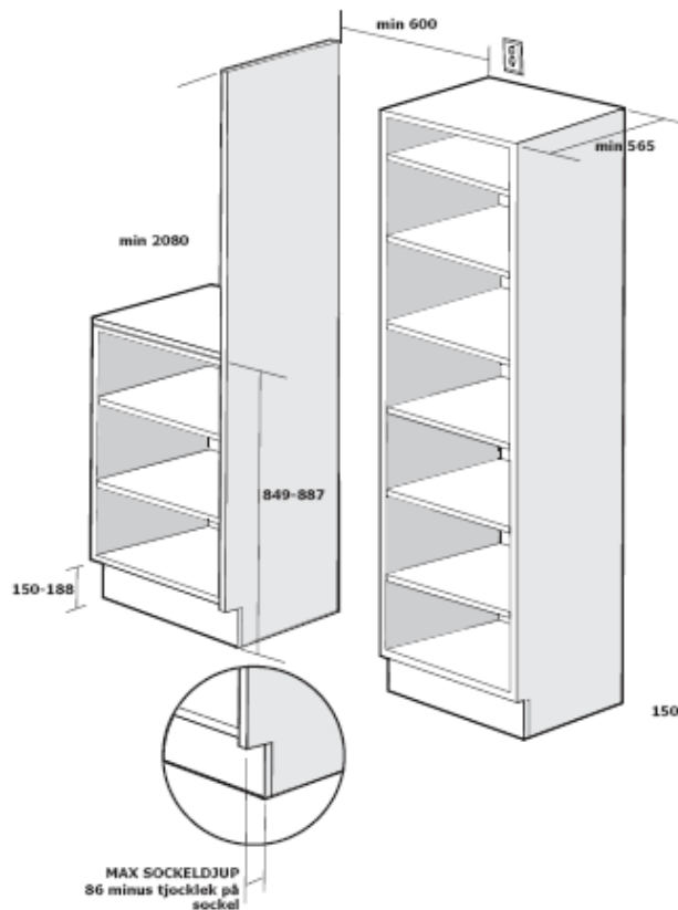
INSTALLATION COMBISKÅP
